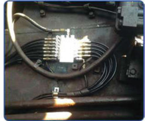
Mono Block Progressive Distributor Performance indicator Type fitted at the bottom of the Dumper to find the exact bearing blockage if any
